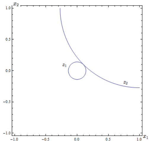
Figure 27: Level curves.
