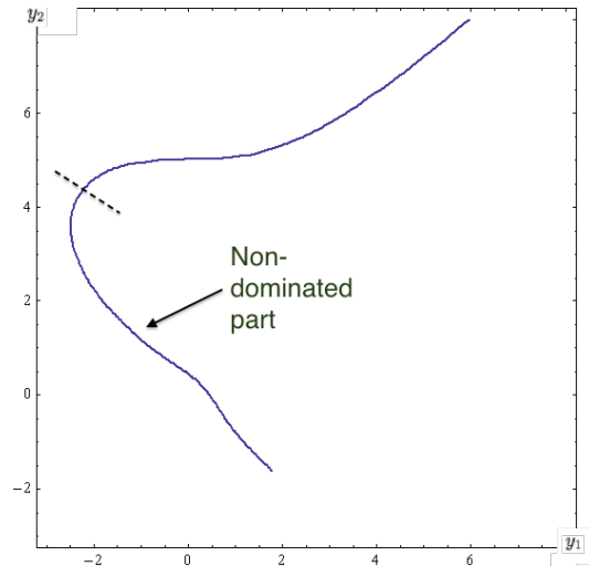
Figure 22: Candidate Set
