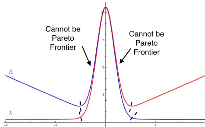
Figure 18: Both functions f_1 and f_2 , when depending only from one variable.
