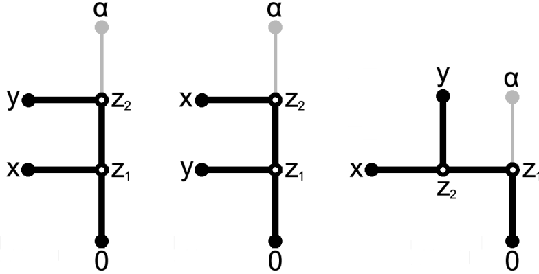
Figure 7: From left to right: the tree diagrams corresponding to the sums \Sigma_1, \Sigma_2 and \Sigma_3 .
