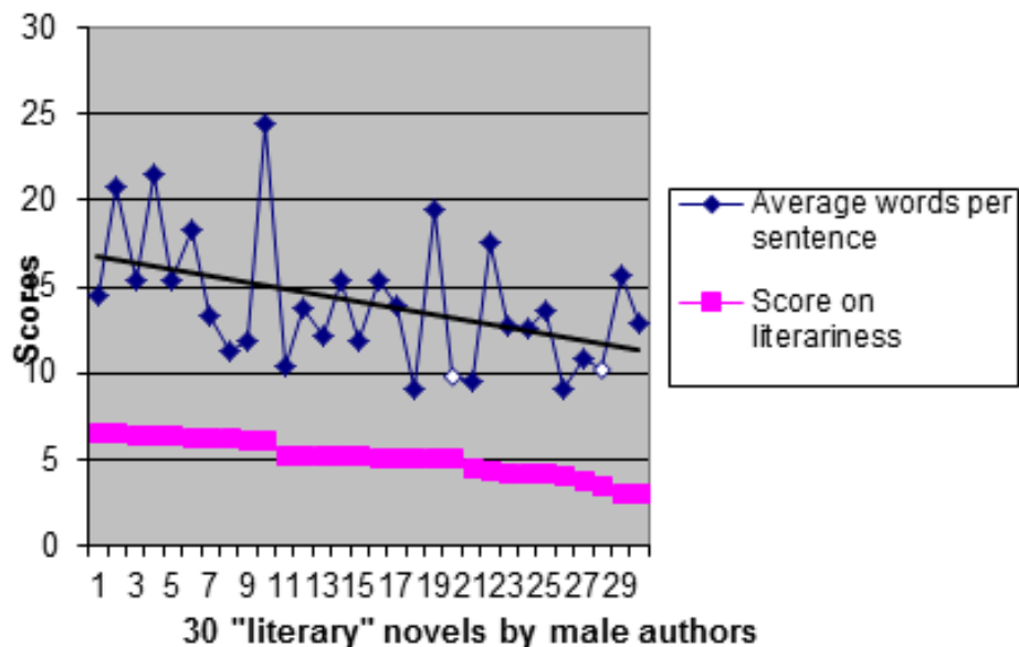
Average words per sentence and score for literariness
