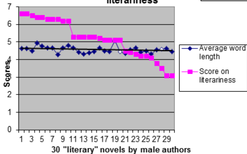
Average word length and score for literariness
