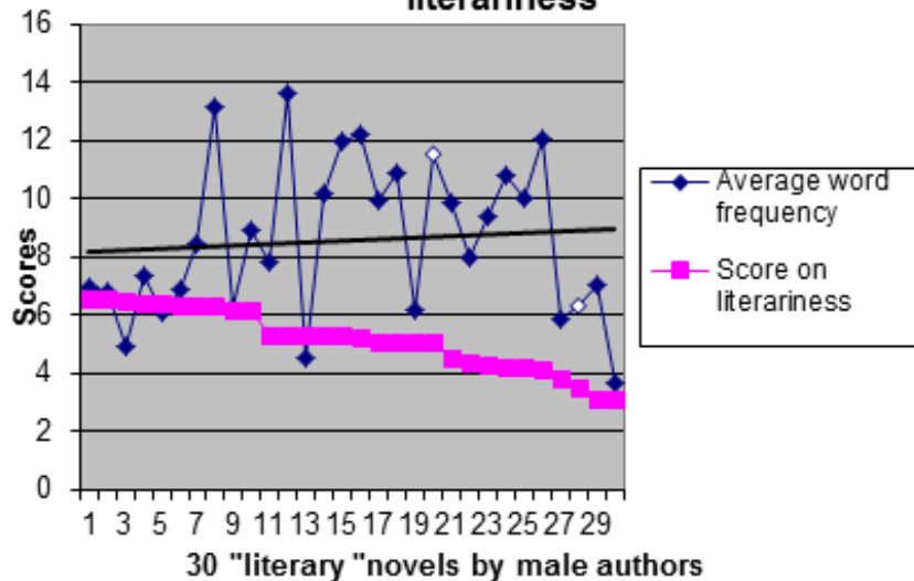
Average word frequency and score for literariness
