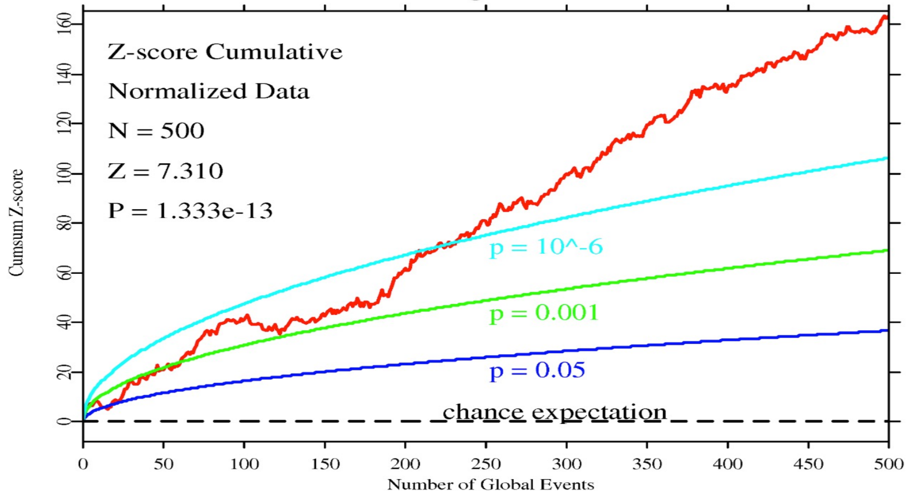
GCP Results, Aug 1998 to Dec 2015
